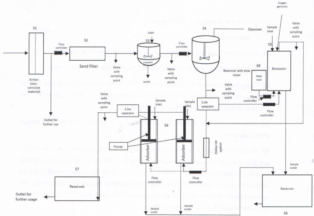
Flow diagram showing tentative setup of pilot plant (tentative)
