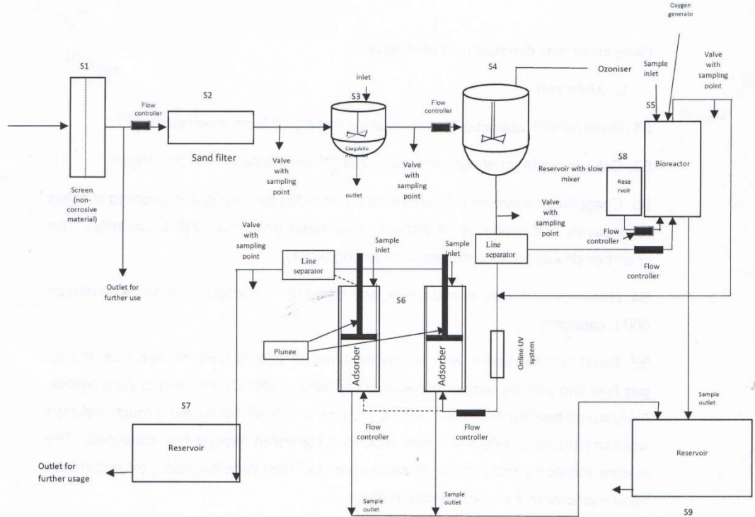
Flow diagram showing tentative setup of pilot plant (tentative)
